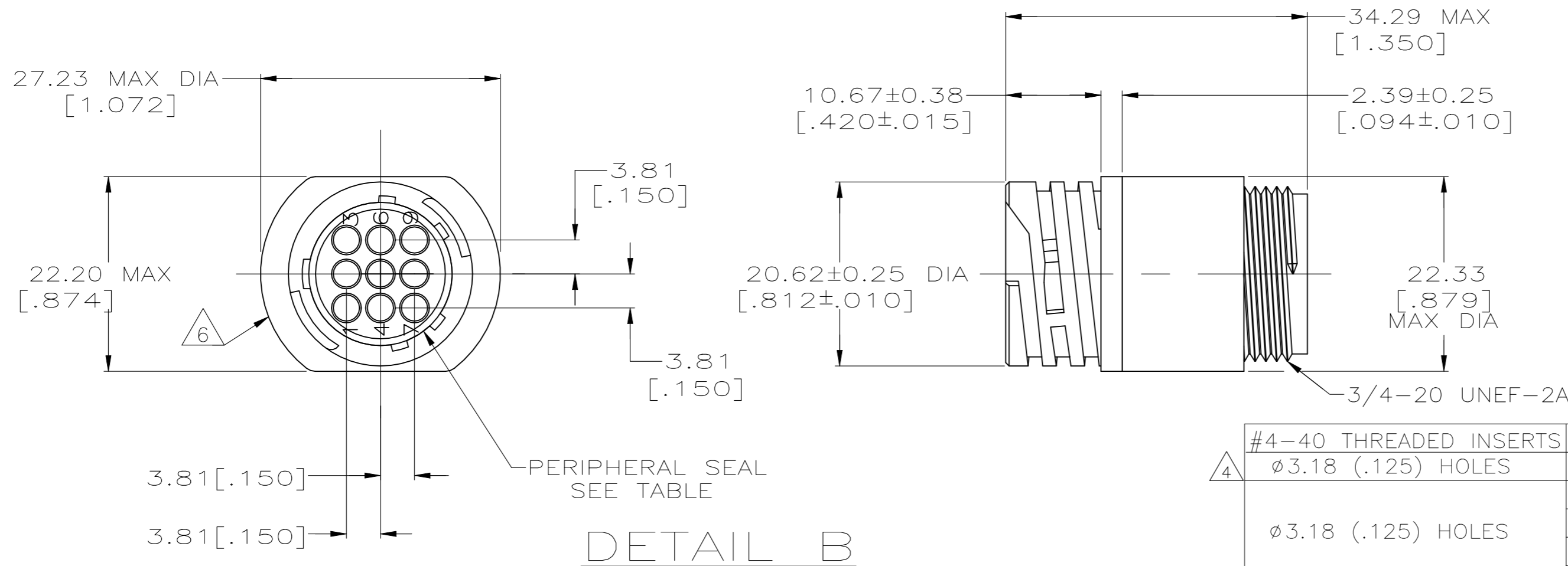
DETAIL A
