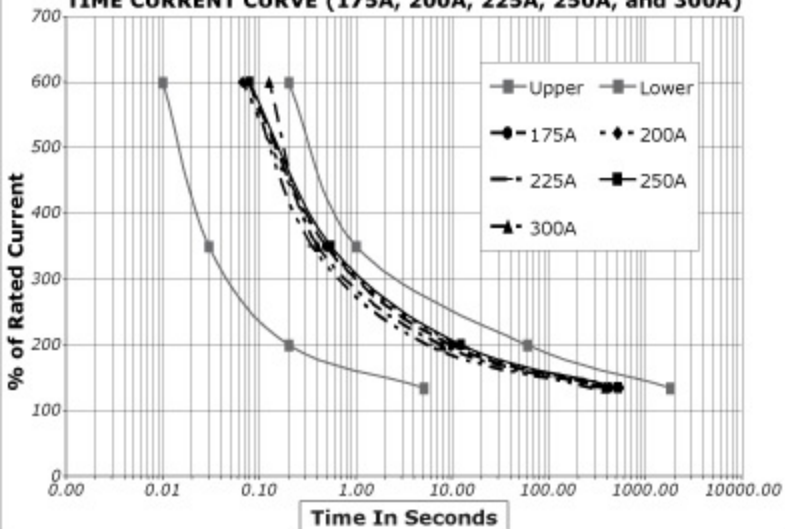
TIME CURRENT CURVE (175A, 200A, 225A, 250A, and 300A)
