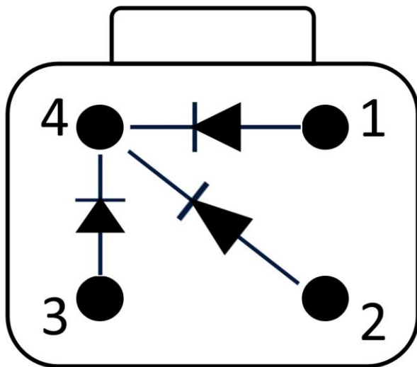
72-0480 Common Cathode Pinout
