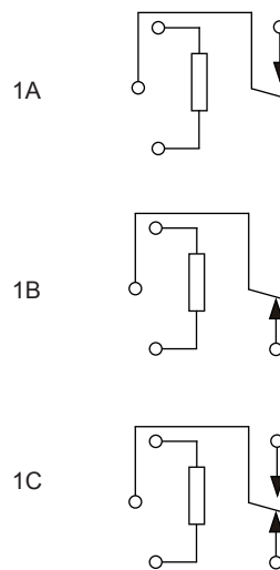
Wiring Diagram (Bottom view)
